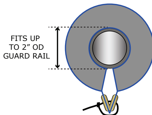
END VIEW INSTALLED
