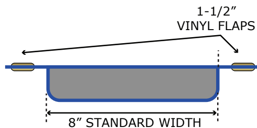
END VIEW FLAT
